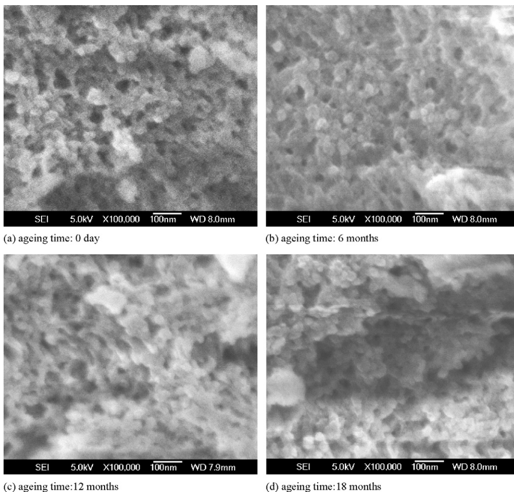
Fig. 6. SEM images of the fresh alum sludge (ageing time: 0 day) and the aged alum sludges (ageing time: 6, 12 and 18 months).
