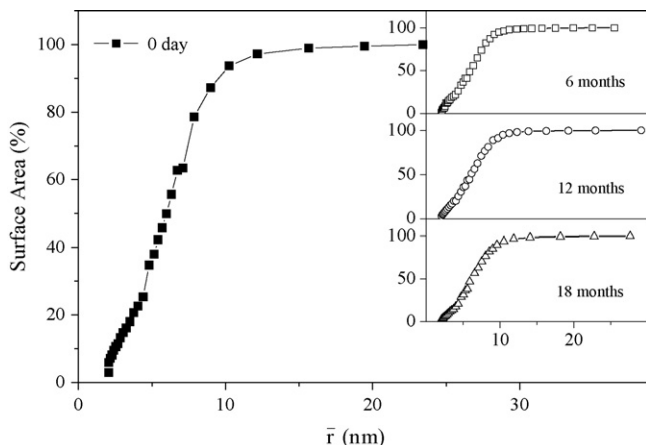
Fig. 7. Mesopore surface area–pore size distribution of the fresh alum sludge (ageing time: 0 day) and the aged alum sludges (ageing time: 6, 12 and 18 months).
